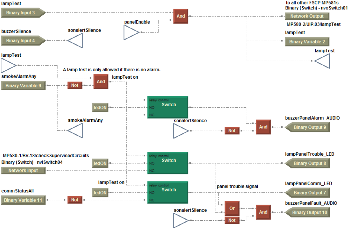
Figure 68. Sample TGP showing lamp test and audio alarm silence routine
